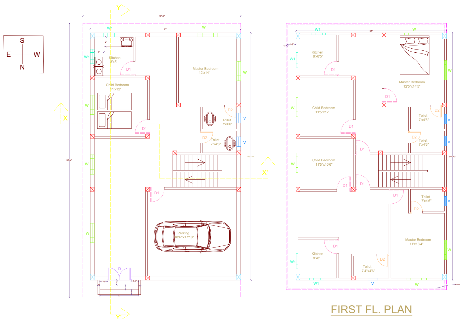
FIRST FL. PLAN
