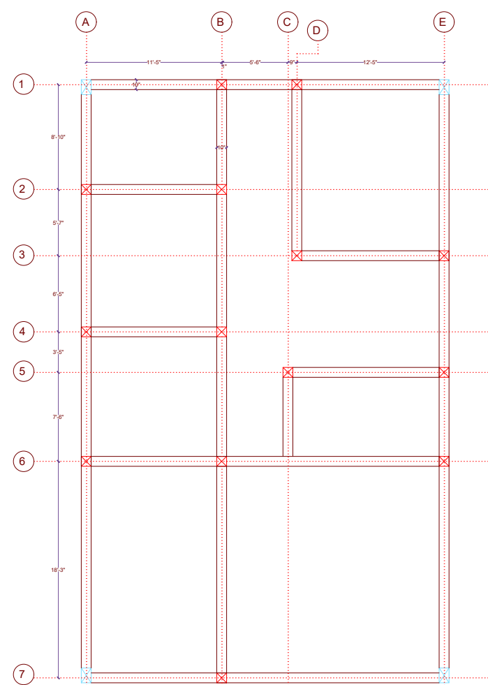
BEAM LAYOUT OF GROUND FL.
