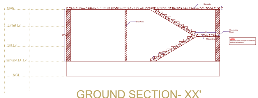
GROUND SECTION- XX'
