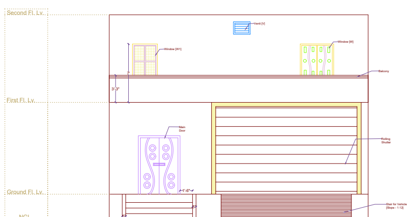
FRONT SIDE ELEVATION
