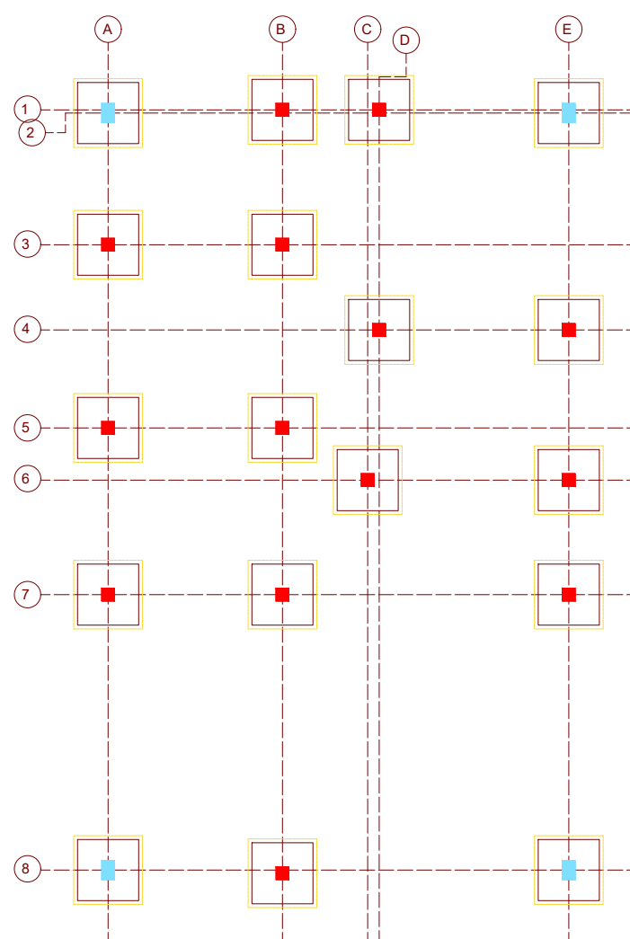
FOOTING LAYOUT WITHOUT SLAB
