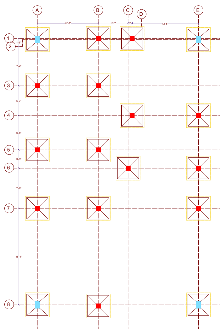
FOOTING LAYOUT WITH SLAB
